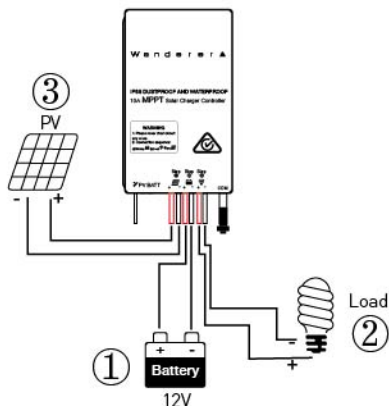
Wiring Diagram
